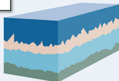
Schematic section through a typical hot dip galvanized coating
